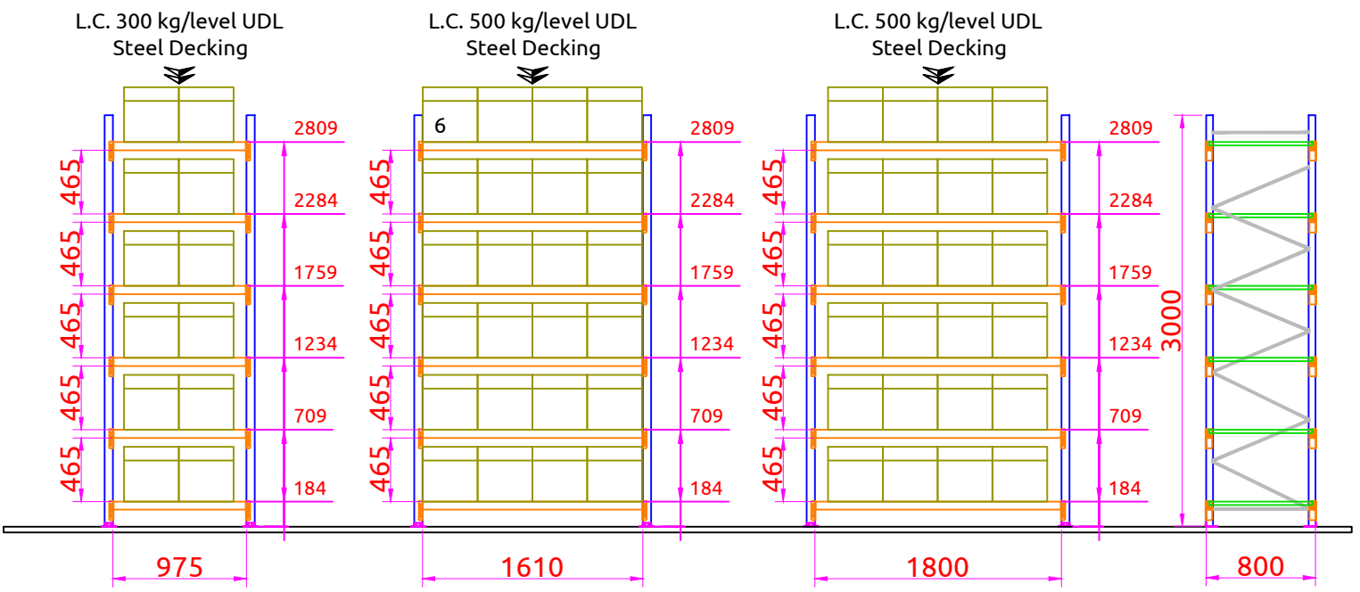
Longspan Racking System TYPICAL FRONT & SIDE ELEVATIONS 69 BAYS
